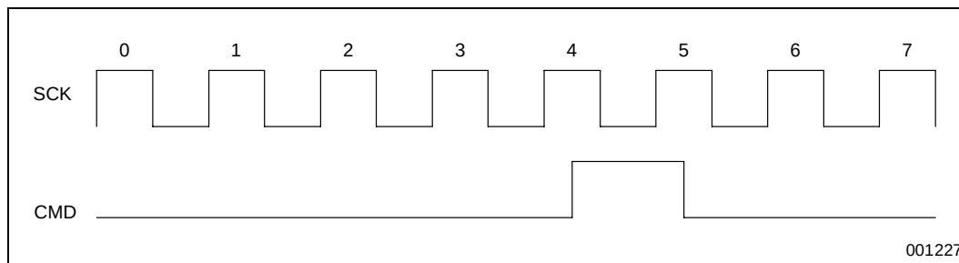
Figure 4-15. SIO Reset Sequence
