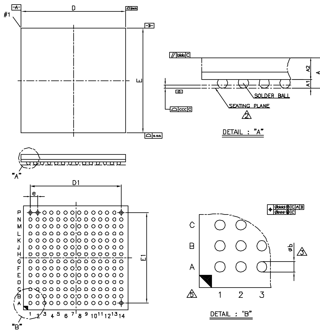
Figure 7. 82573 Mechanical Specifications
