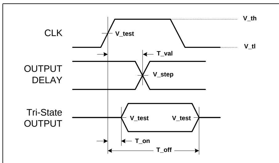
Figure 25. Output Timing Measurement Conditions
