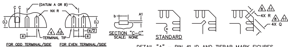
DETAIL "A" — PIN #1 ID AND TIEBAR MARK FIGURES
