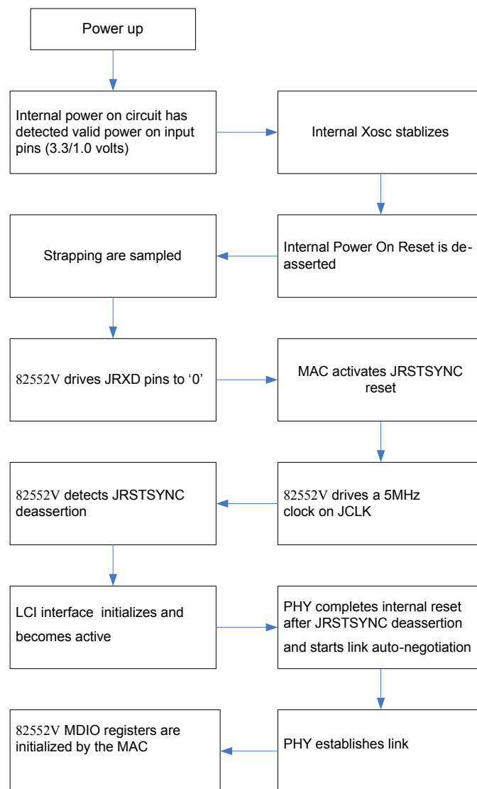
Figure 4. Power Up Sequence Flowchart
