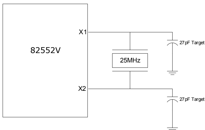
Figure 11. Crystal Connection Diagram
