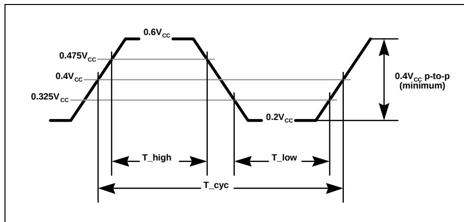
Figure 20. PCI Clock Waveform
