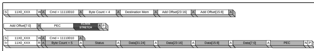
Figure 2-2. DWord Memory Read Protocol (SMBus Block Write/Block Read, PEC Enabled)
