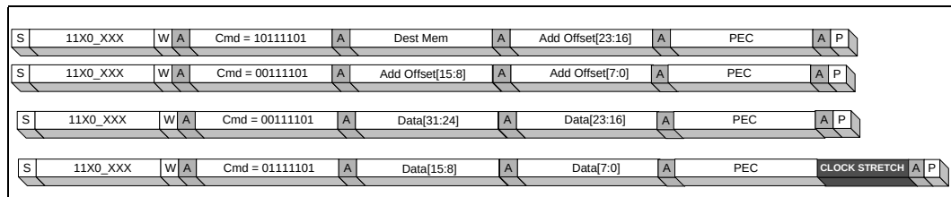
Figure 2-9. Word Configuration Write Protocol (SMBus Byte Write, PEC Enabled)
