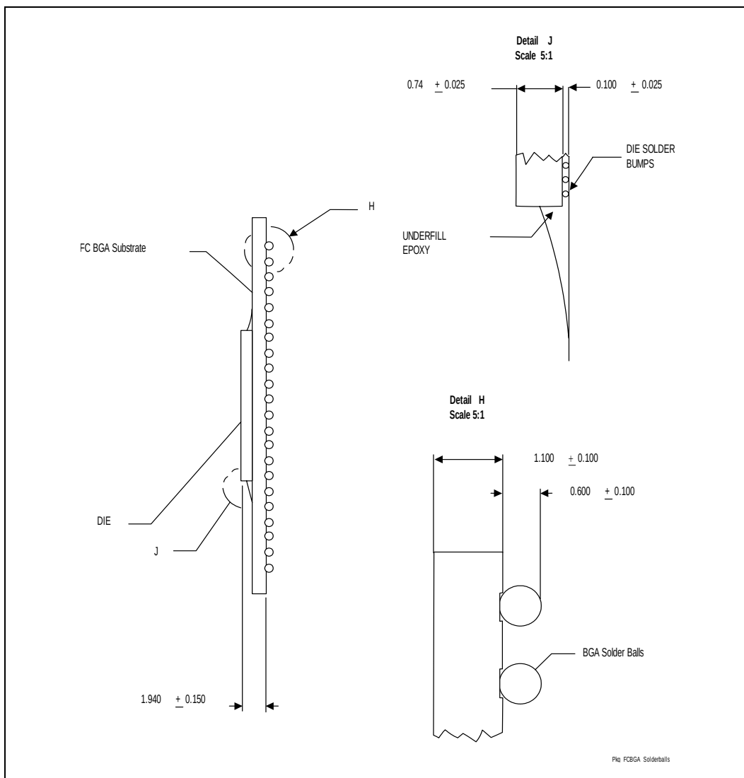
Figure 6-3. Side View – Intel® 6700PXH 64-bit PCI Hub 567-Ball FCBGA Package Dimensions
