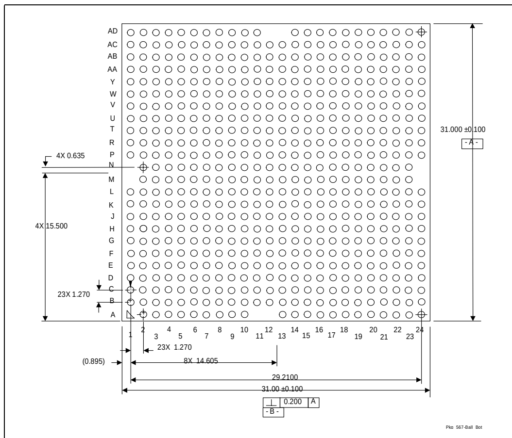
Figure 6-2. Bottom View – Intel® 6700PXH 64-bit PCI Hub 567-Ball FCBGA Package Dimensions
