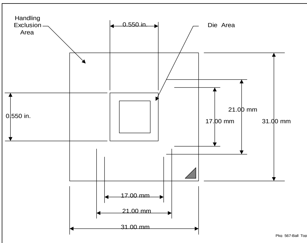
Figure 6-1. Top View – Intel® 6700PXH 64-bit PCI Hub 567-Ball FCBGA Package Dimensions
