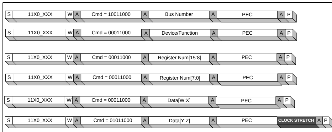
Figure 2-9. Word Configuration Write Protocol (SMBus Byte Write, PEC Enabled)
