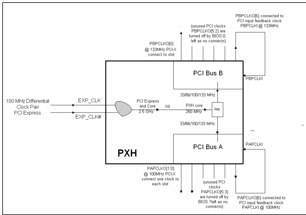
Figure 2-12. Intel® 6700PXH 64-bit PCI Hub Clocking Diagram
