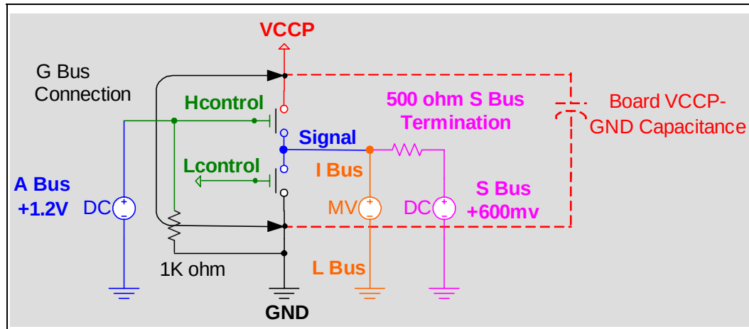
Figure 4-3. Instrument Setup For High Side Switch
