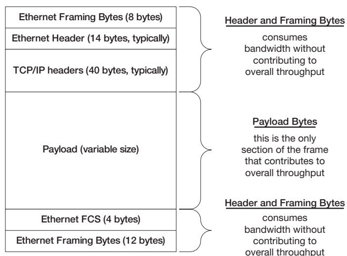
Figure 1. Typical TCP/IP Ethernet Frame
