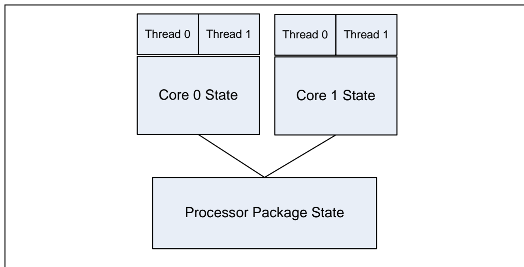
Figure 4-1. Idle Power Management Breakdown of the Processor Cores
