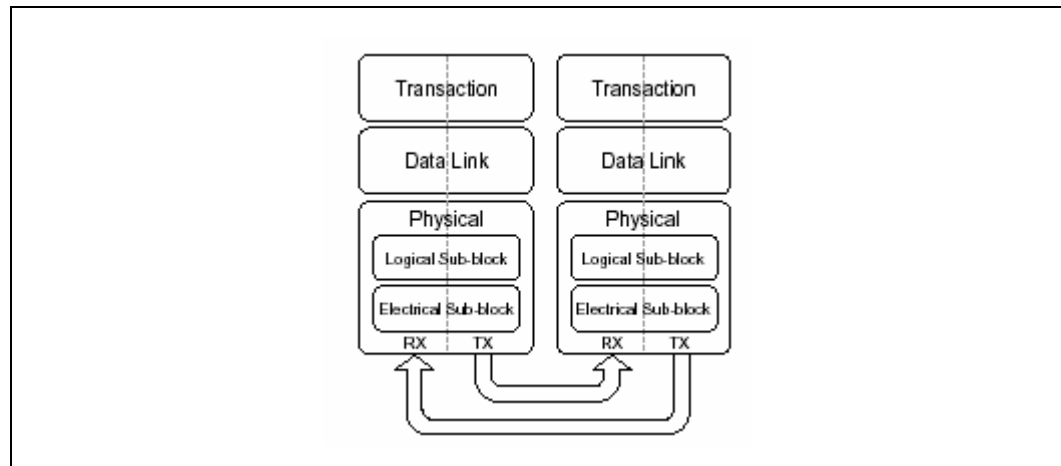
Figure 2-3. PCI Express* Layering Diagram
