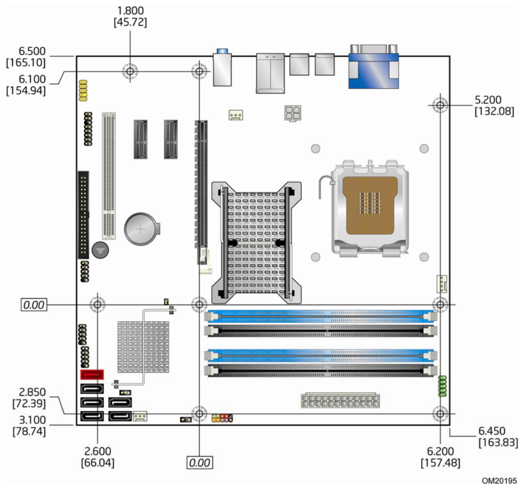
Figure 15. Board Dimensions
