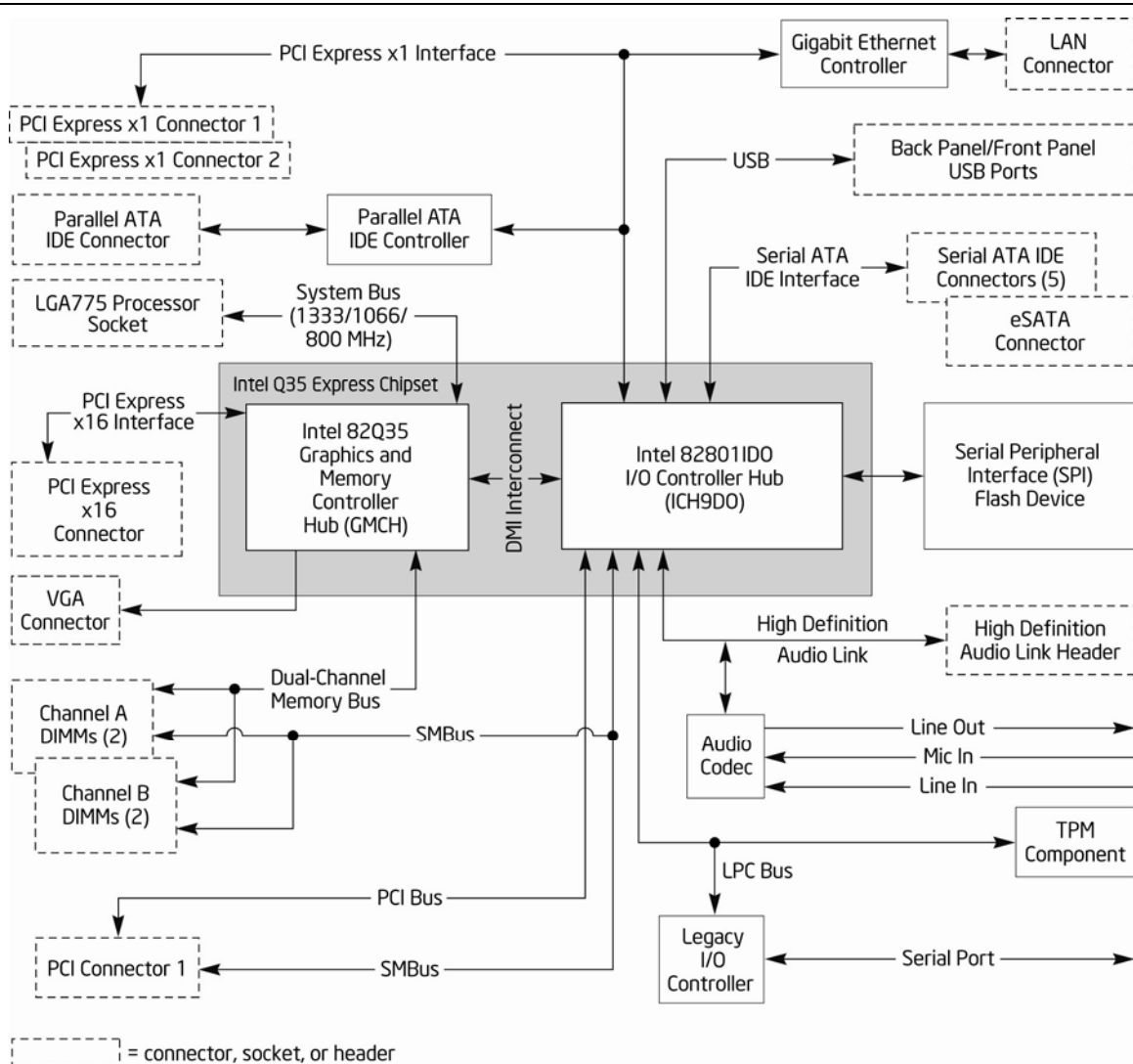
Figure 2. Block Diagram
