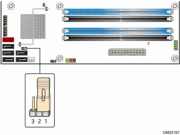
Figure 14. Location of the Jumper Block
