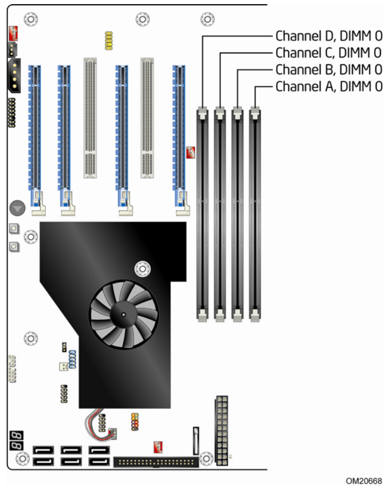
Figure 3. Memory Channel and DIMM Configuration
