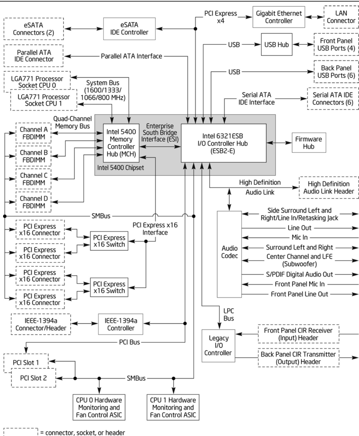
Figure 2. Block Diagram
