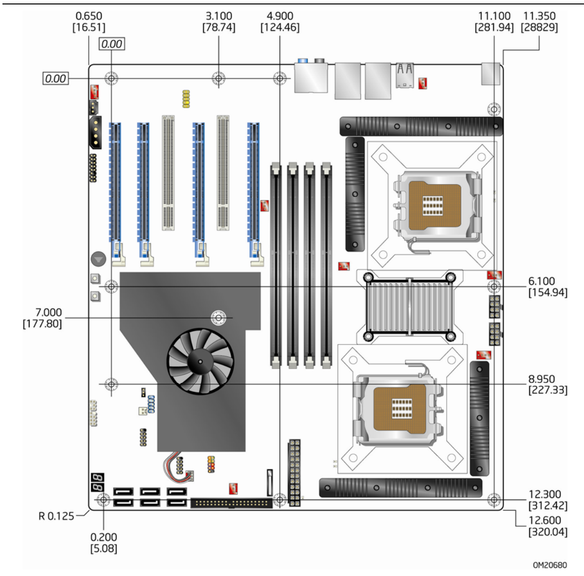
Figure 16. Board Dimensions
