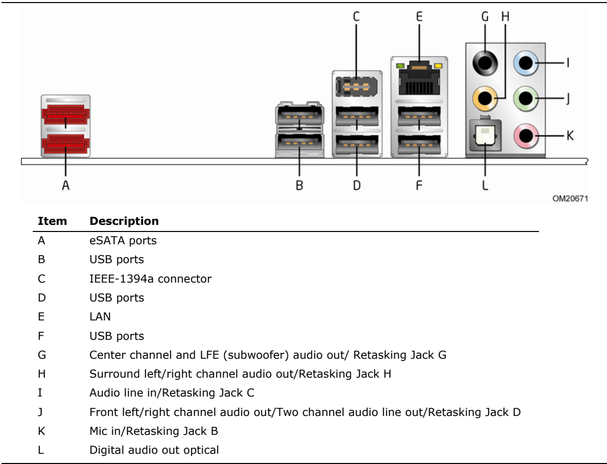
Figure 10. Back Panel Connectors
