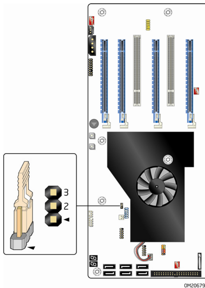
Figure 15. Location of the Jumper Block
